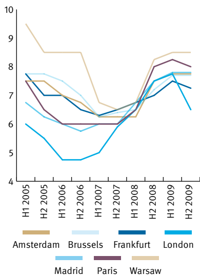
Figure 4 Logistics prime yield movements %
